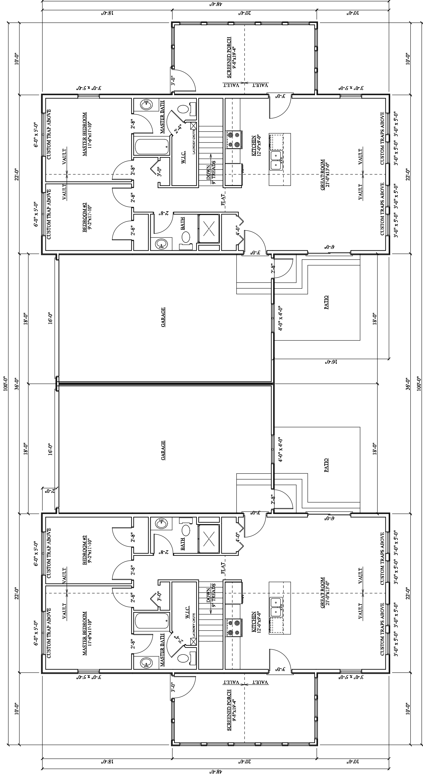
MAIN FLOOR PLAN SCALE: 1/4" = 1'-0"
